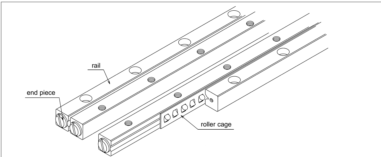
Figure H-1 Slide Way Structure
