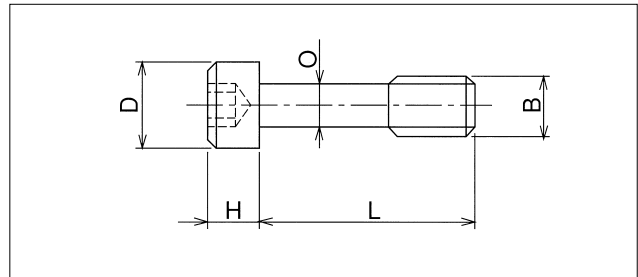
Figure H-9 BT type Special Bolt
