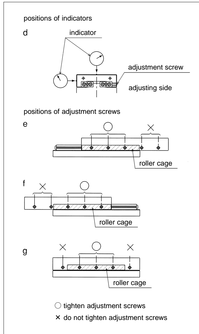
Figure H-8 Installation Method (2)
