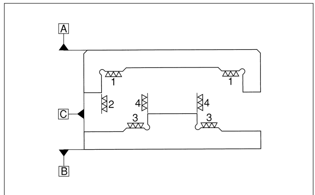
Figure H-6 Accuracy of Mounting Surfaces
