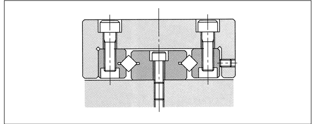
Figure H-5 SVW Type Slide Way
