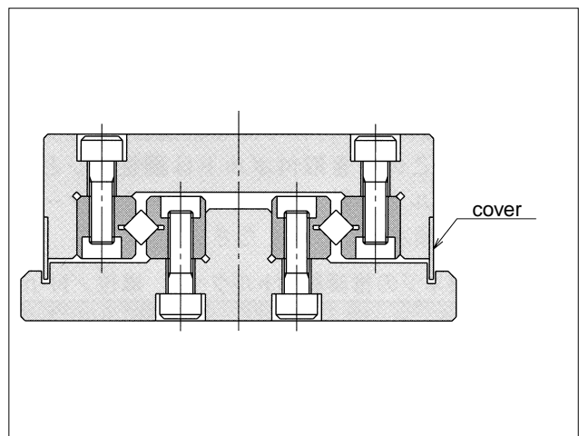
Figure H-10 Use of Cover to Prevent Dust
