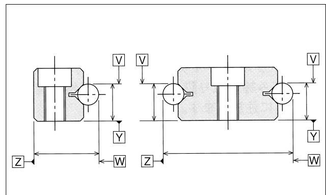
Figure H-3 Accuracy Measurement Method
