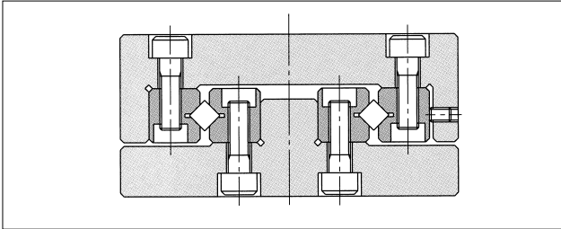
Figure H-4 SV Type Slide Way
