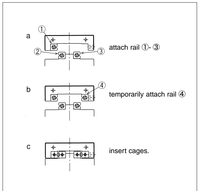
Figure H-7 Installation Method (1)
